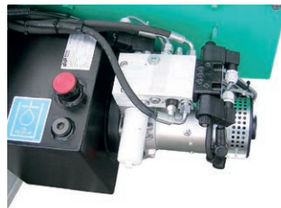
Hydraulikaggregat
